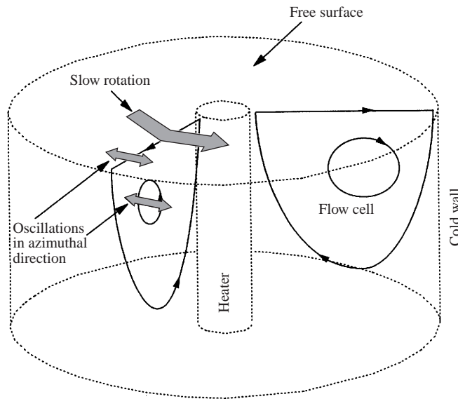
FIGURE 11. Sketch of the oscillatory flow field.
